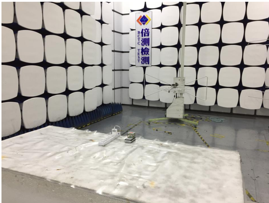
Spurious emissions
