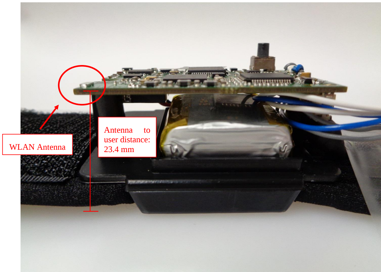
Photo 3: Antenna location (Side view, cover removed)
