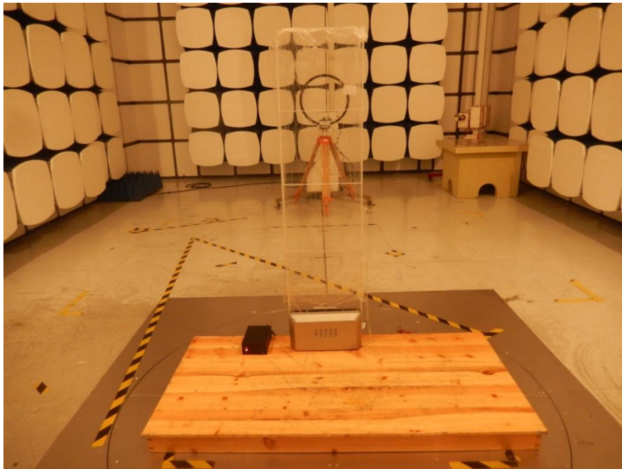
FAP radiation below 30MHz
