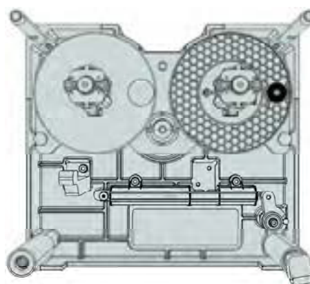
Left-hand cassette
