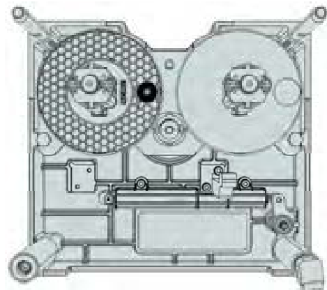
Right-hand cassette
