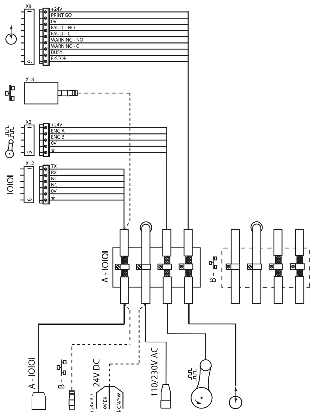
Electrical Diagram 10073532
