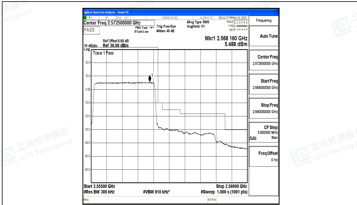
Band7_15MHz_QPSK_21375_75RB#0
