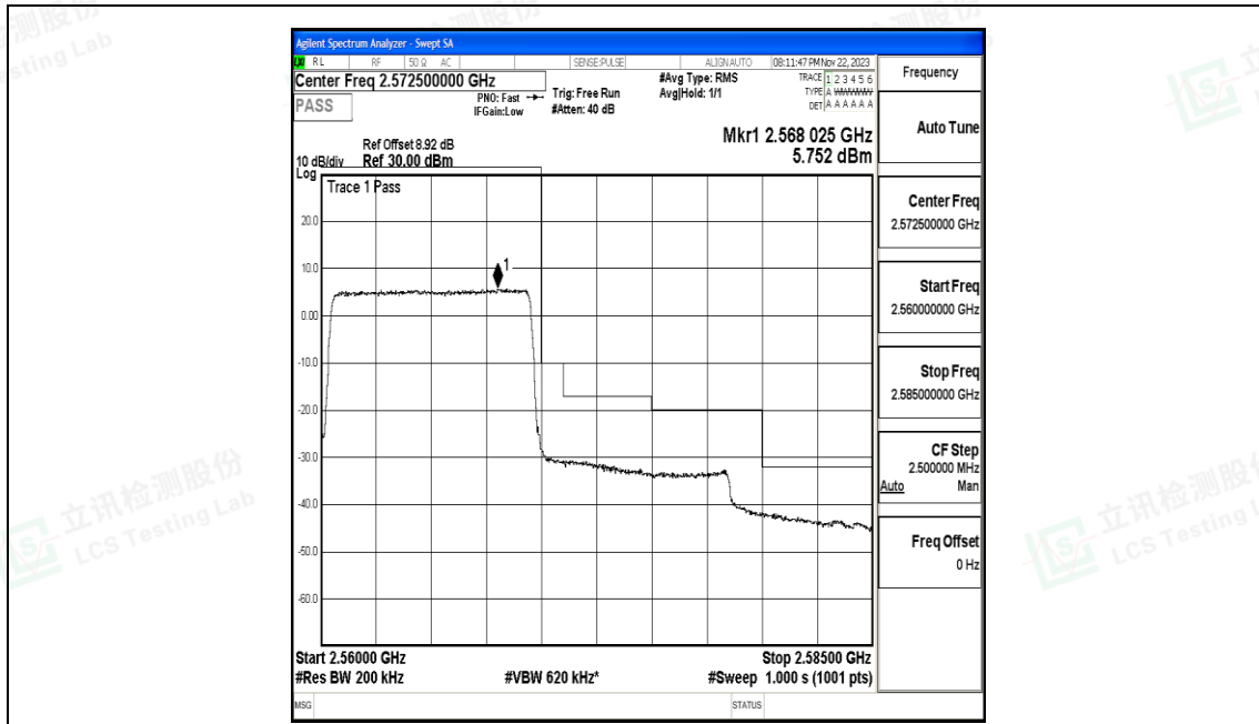
Band7_10MHz_QPSK_21400_50RB#0
