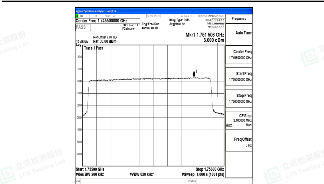
Band4_20MHz_16QAM_20300_100RB#0
