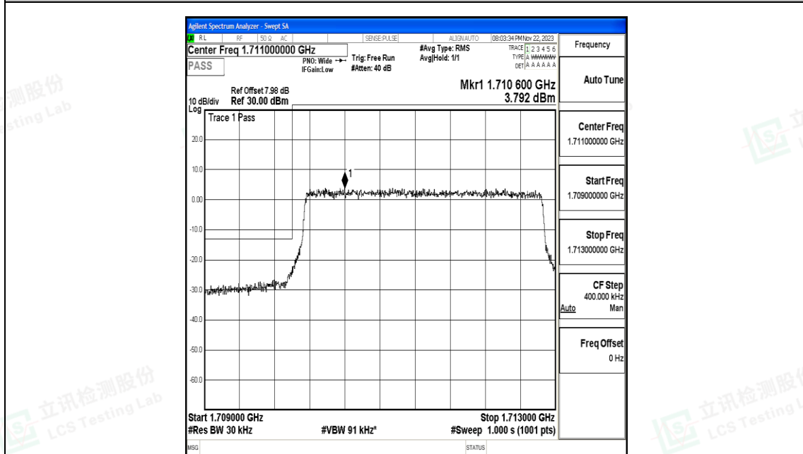
Band4_3MHz_16QAM_19965_15RB#0
