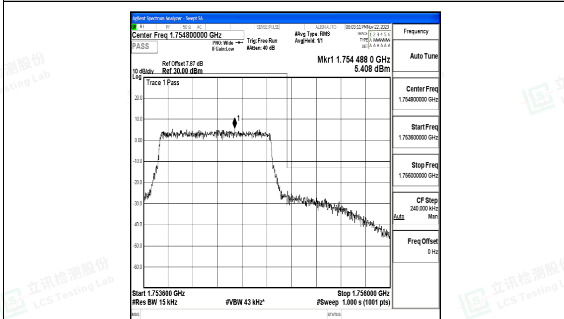
Band4_1.4MHz_16QAM_20393_6RB#0
