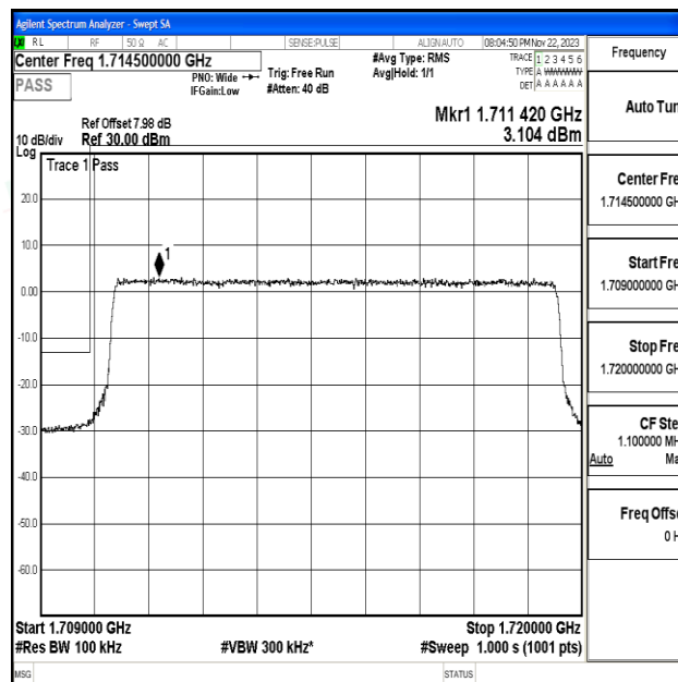
Band4_10MHz_16QAM_20000_50RB#0
