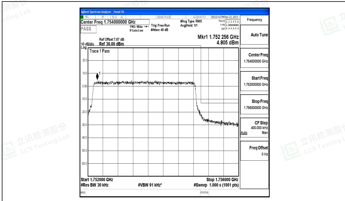
Band4_3MHz_QPSK_20385_15RB#0
