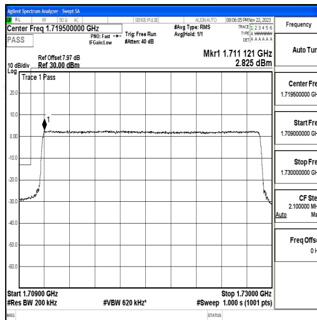
Band4_20MHz_16QAM_20050_100RB#0
