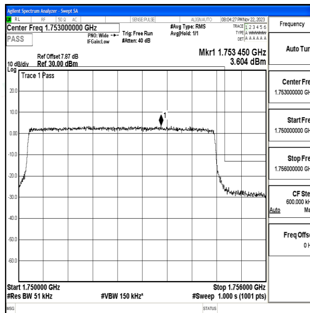
Band4_5MHz_16QAM_20375_25RB#0
