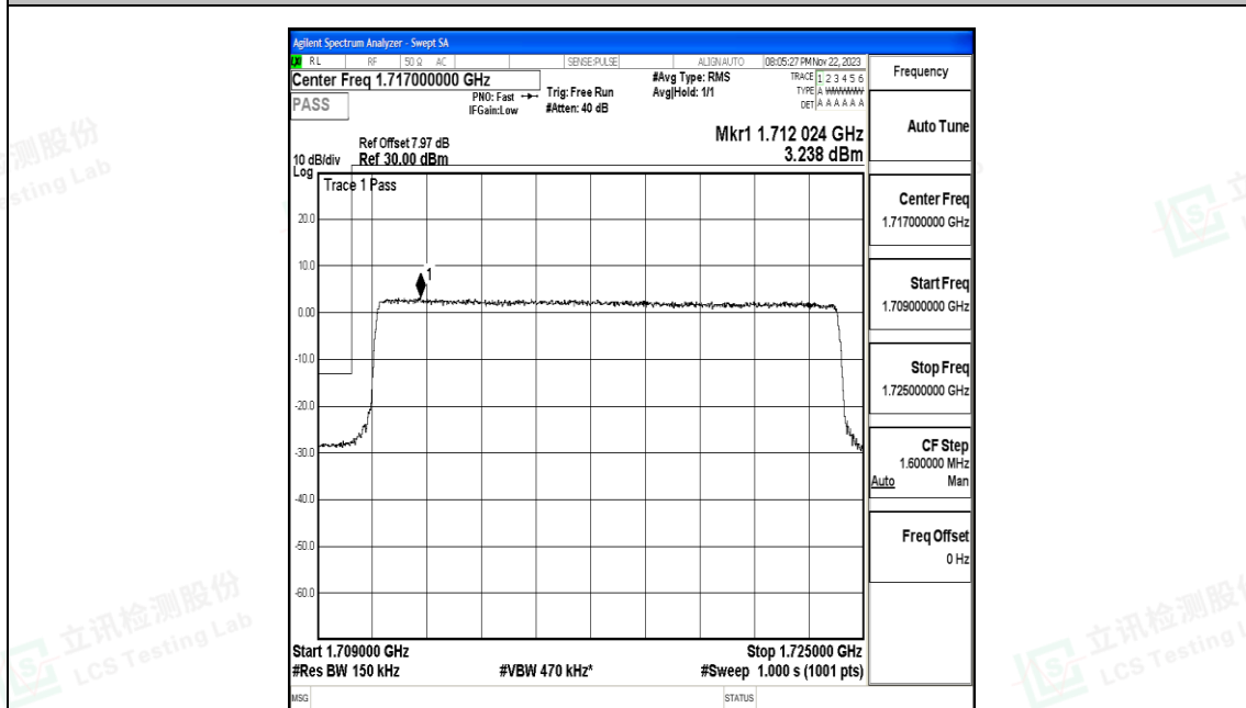
Band4_15MHz_16QAM_20025_75RB#0
