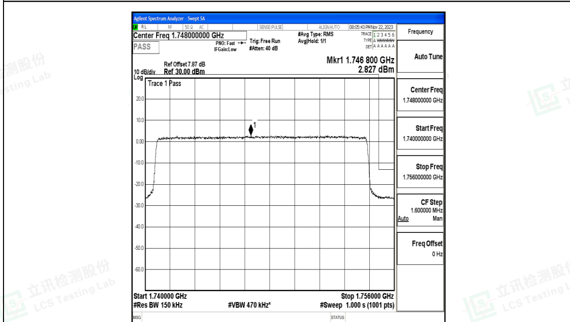
Band4_15MHz_16QAM_20325_75RB#0
