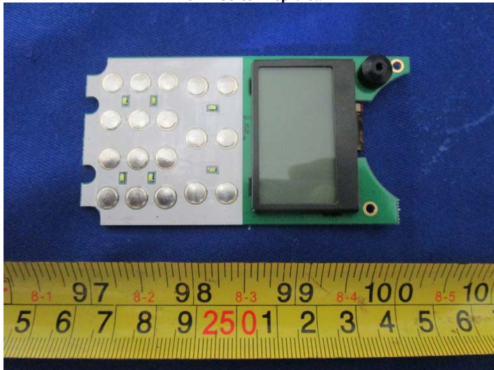
EUT – Screen Top View
