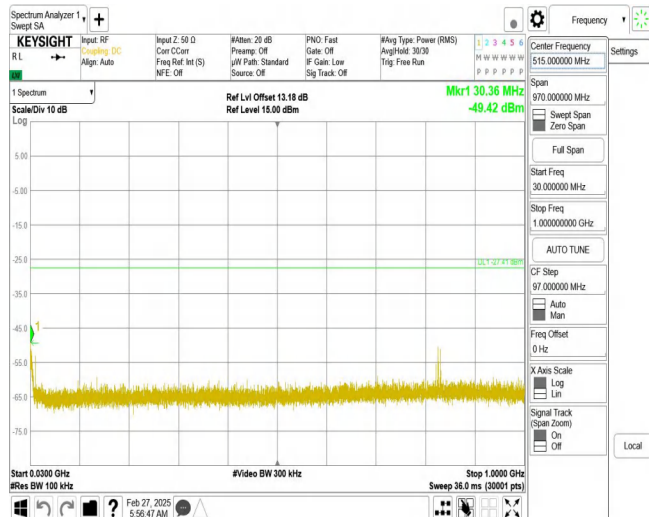
11N40SISO_Ant1_2437_30~1000
