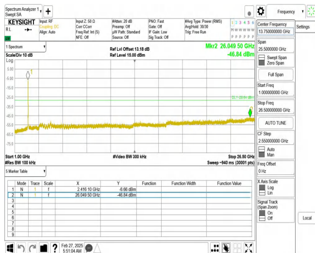
11N40SISO_Ant1_2422_1000~26500
