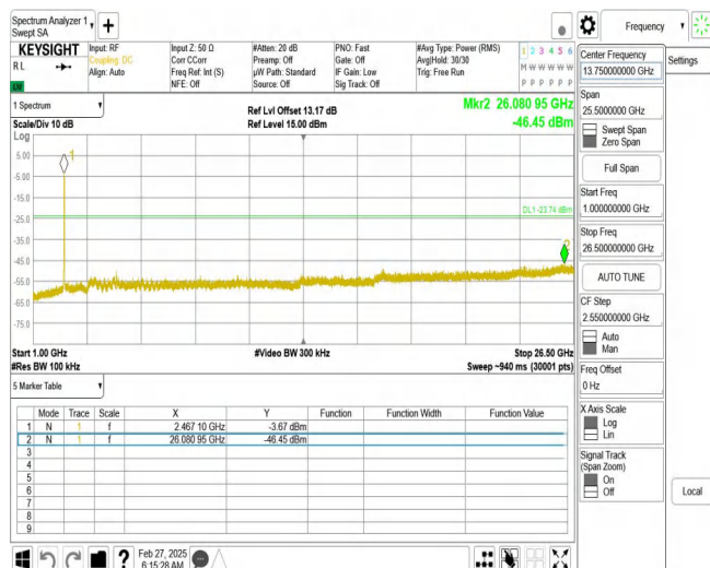
11N20SISO_Ant1_2462_1000~26500
