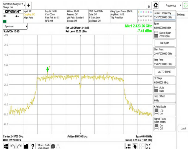
11N40SISO_Ant1_2437_0~Reference
