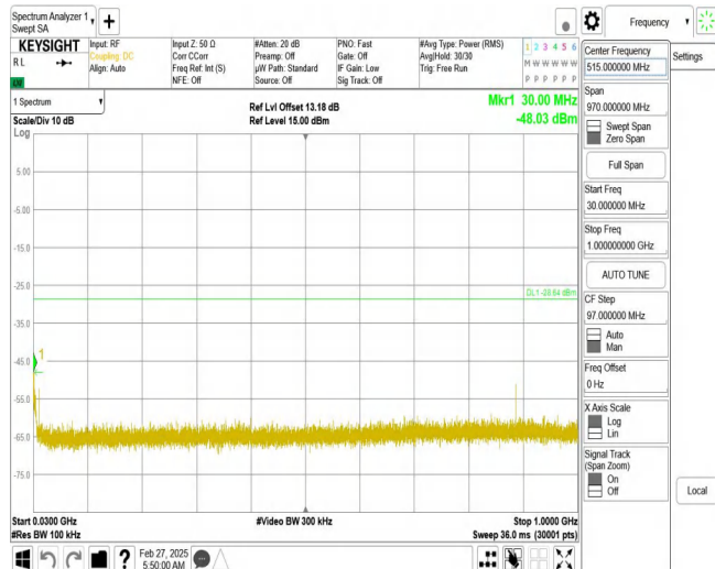
11N40SISO_Ant1_2422_30~1000
