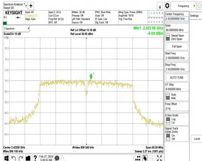
11N40SISO_Ant1_2422_0~Reference
