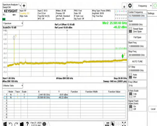
11N40SISO_Ant1_2437_1000~26500
