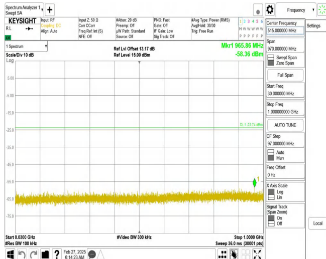
11N20SISO_Ant1_2462_30~1000
