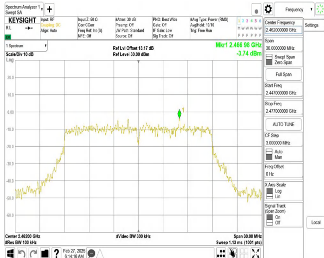
11N20SISO_Ant1_2462_0~Reference
