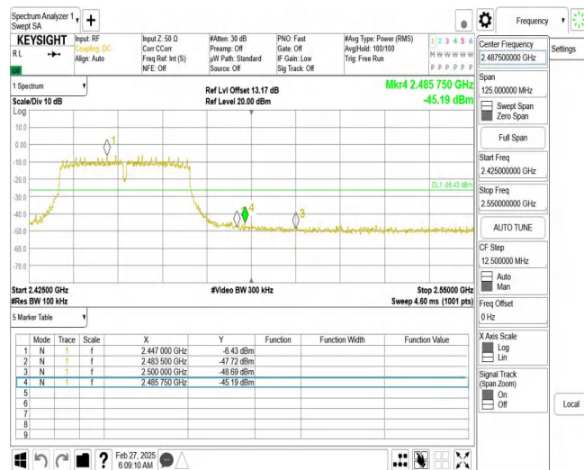
11N40SISO_Ant1_High_2452
