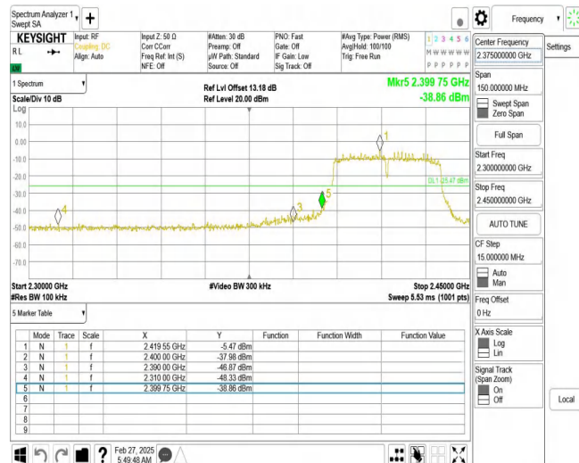
11N40SISO_Ant1_Low_2422
