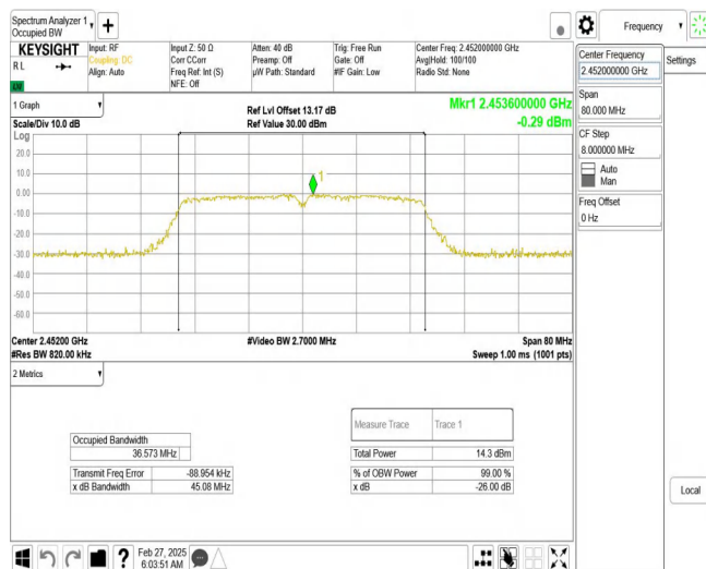
11N40SISO_Ant1_2452
