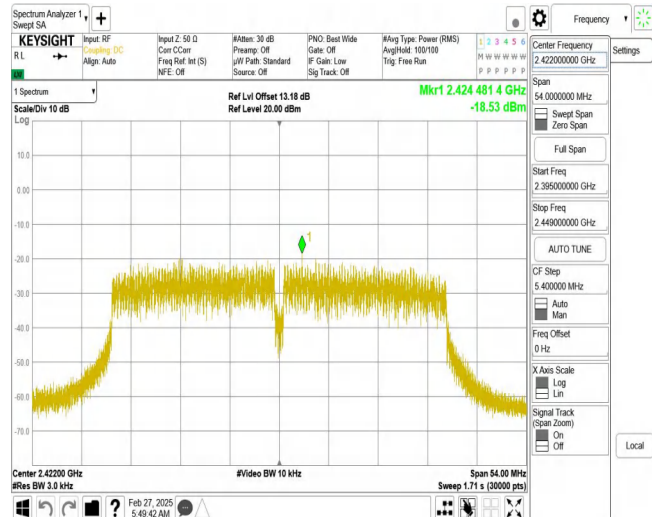
11N40SISO_Ant1_2422
