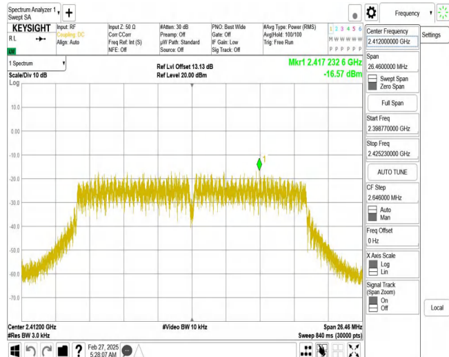
11N20SISO_Ant1_2412
