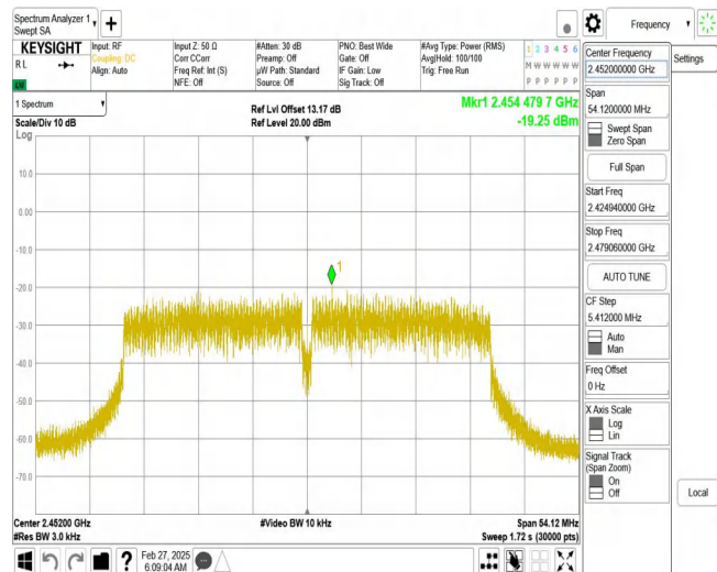
11N40SISO_Ant1_2452
