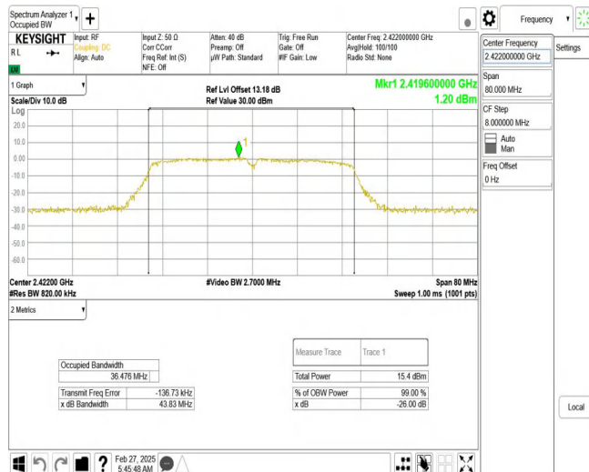
11N40SISO_Ant1_2422
