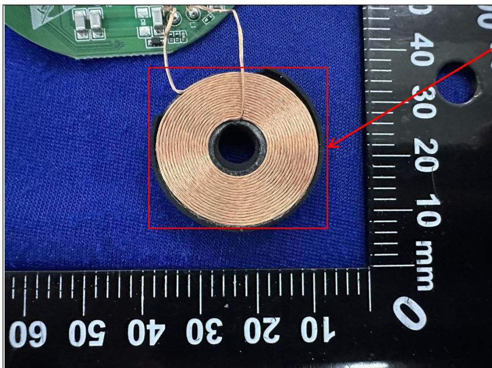
WPT Antenna
