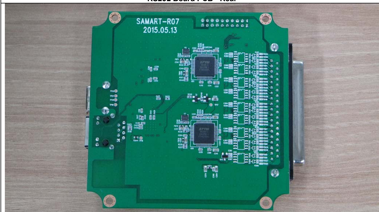
RS232 Board PCB - Rear
