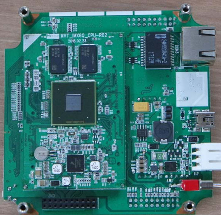
Main board - Front
