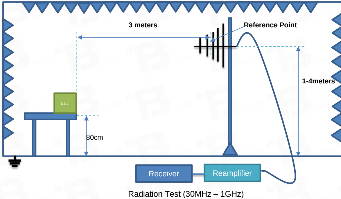
Test Setup 1
