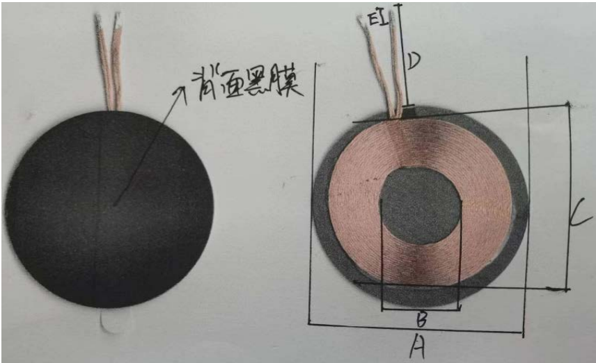
外形图/OUTSIDE DIAGRA
