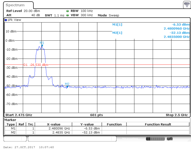
8-DPSK: Band Edge-High Channel (Hopping Mode)
