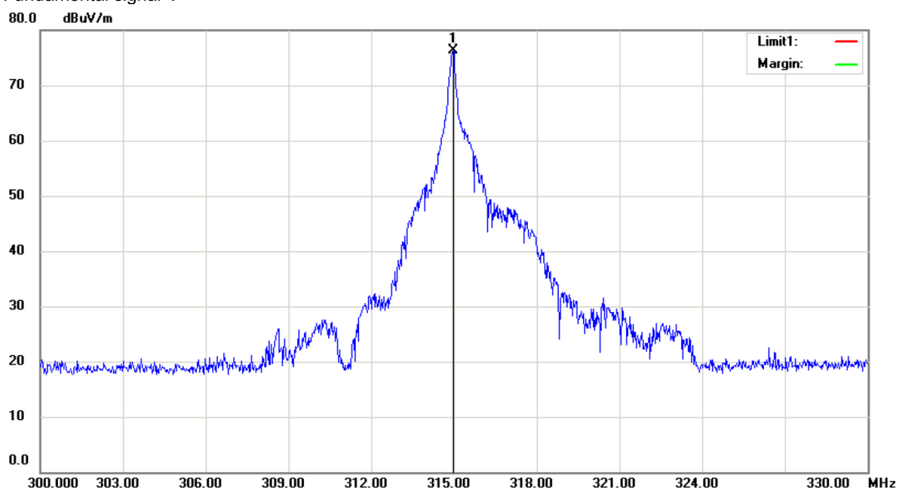
Fundamental signal-V
