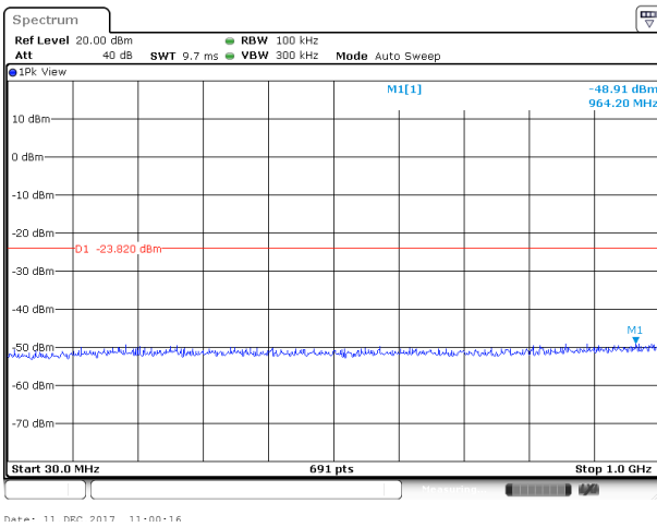
GFSK on channel 78
