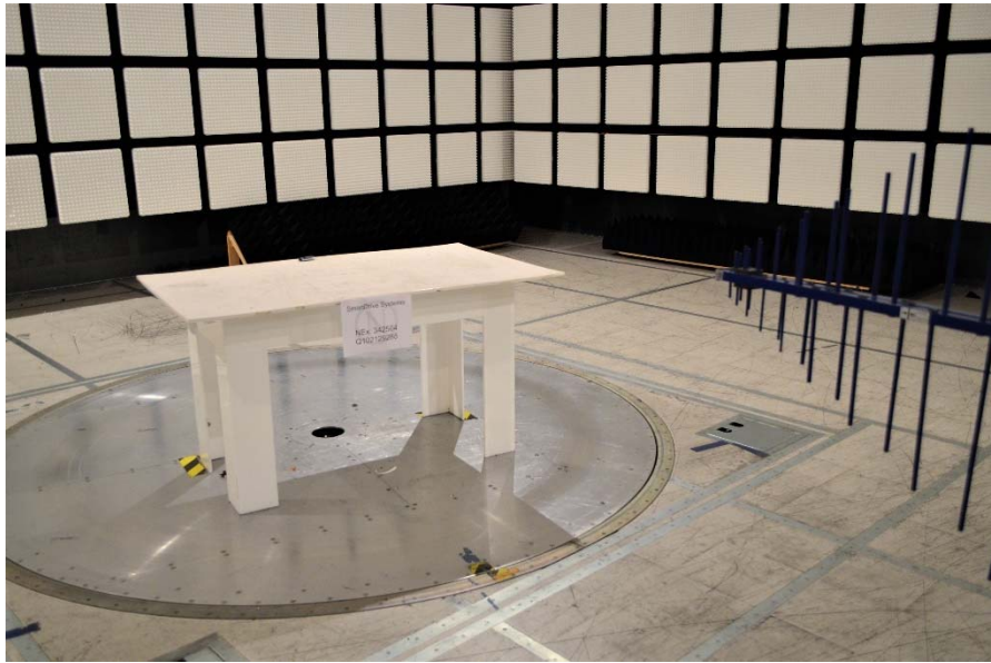
Figure 1.1-1: 30MHz-1GHz (Front View)
