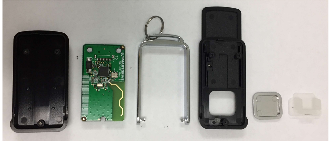
Internal Exploded View, Top PCB
