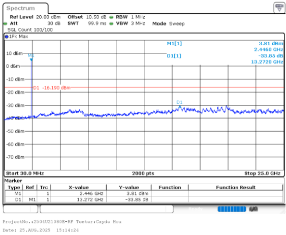
BLE_1M_Middle_Channel
