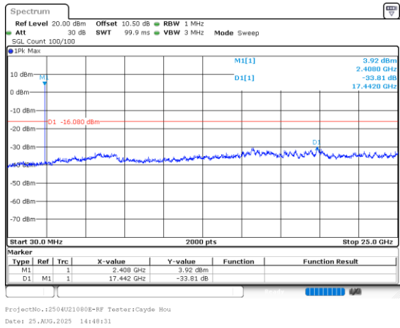
BLE_1M_Low_Channel
