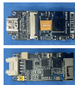
ESP32 TimerCAM
