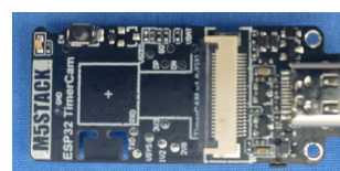
ESP32 TimerCAM
