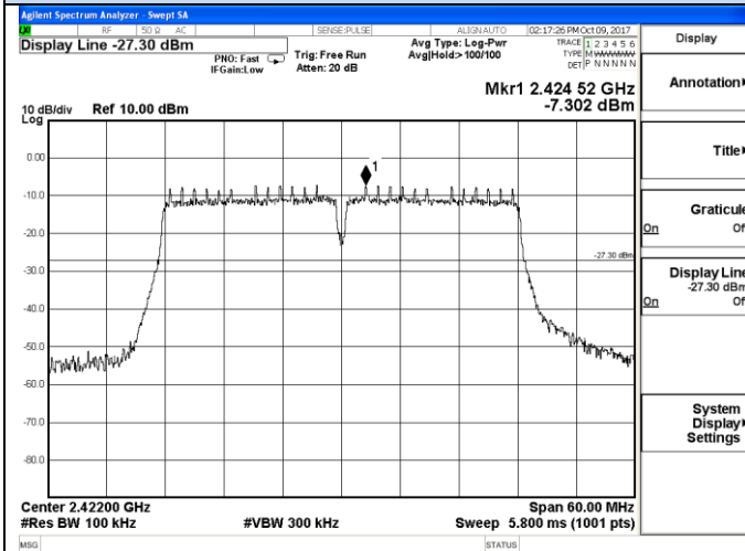
IEEE 802.11n(HT40)-Low channel Reference
