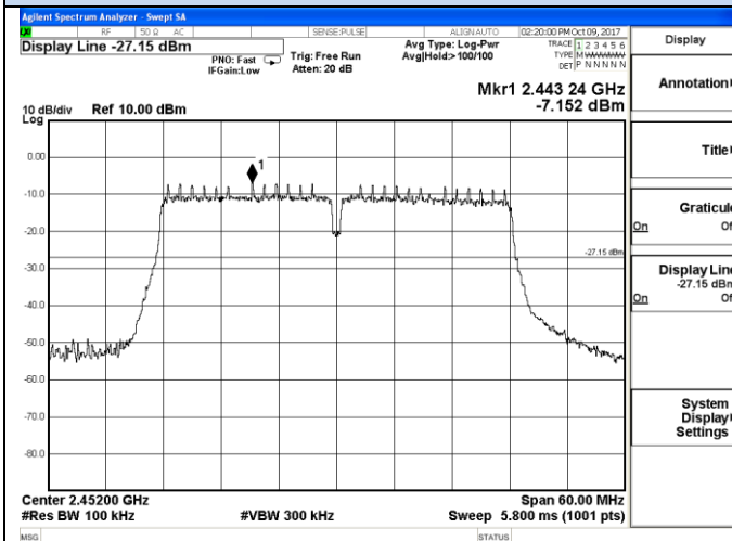
IEEE 802.11n(HT40)-High channel Reference
