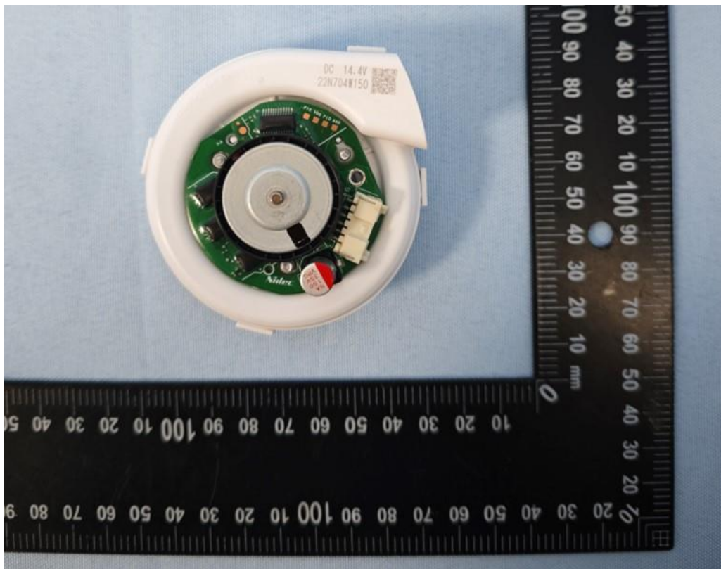
Alternative suction motor 22N704W150
