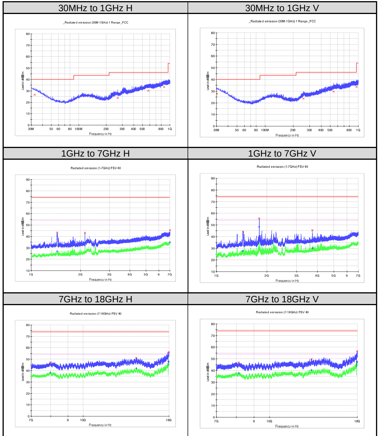
Figure 17: Radiated Spurious Emission, g-2462MHz
