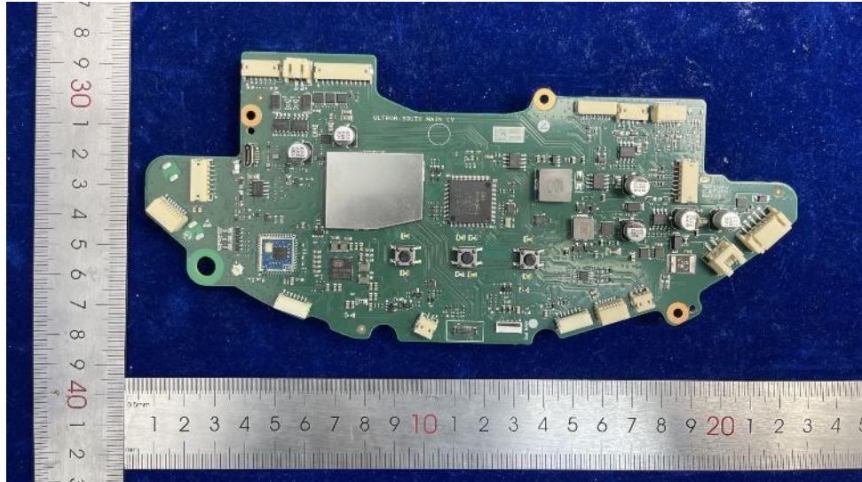
Main board (use new charging IC)
