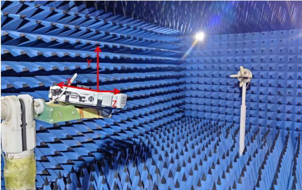
Antenna Set up Photo
