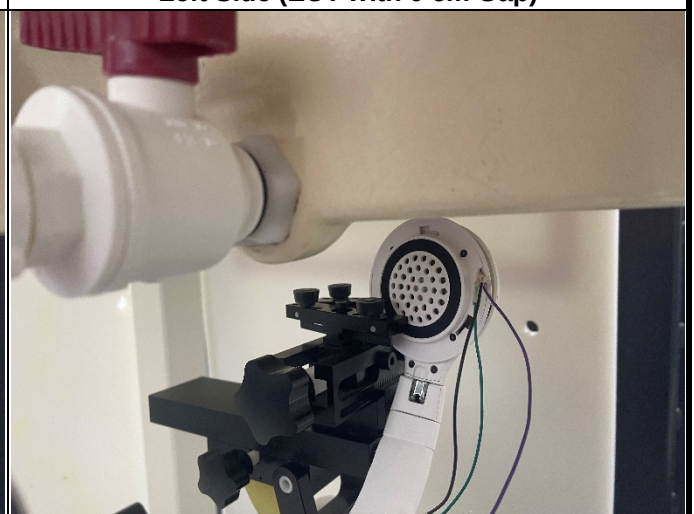
Bottom Side (EUT with 0 cm Gap)
