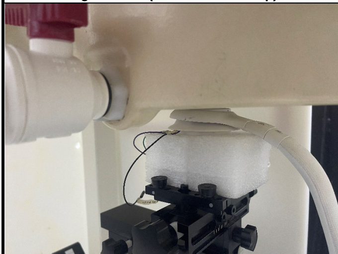
Rear Face (EUT with 0 cm Gap)
