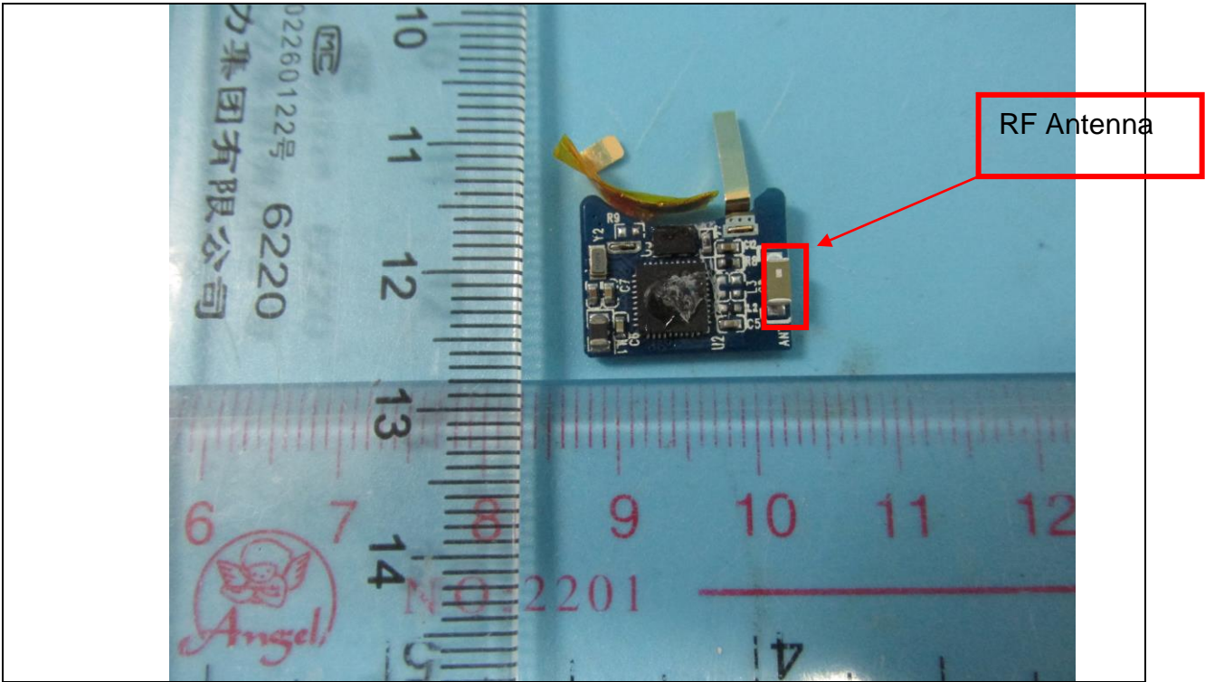
Details of: PCB view 3 (For models C-XT001-B and C-XF001-B)
