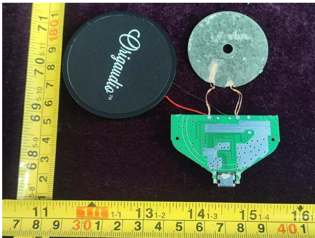
FIGURE 9 LIGHT UP MAGNETIC WIRELESS CHARGER (98371) MAINBOARD BACK
