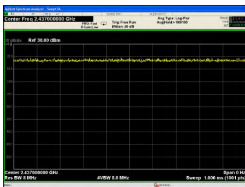
802.11g
