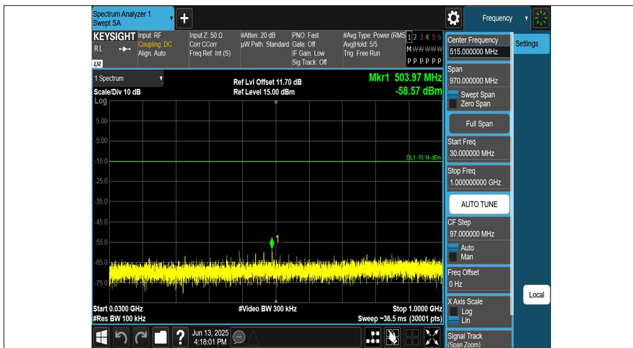
GFSK-Ant1-2436-30~1000-PASS
