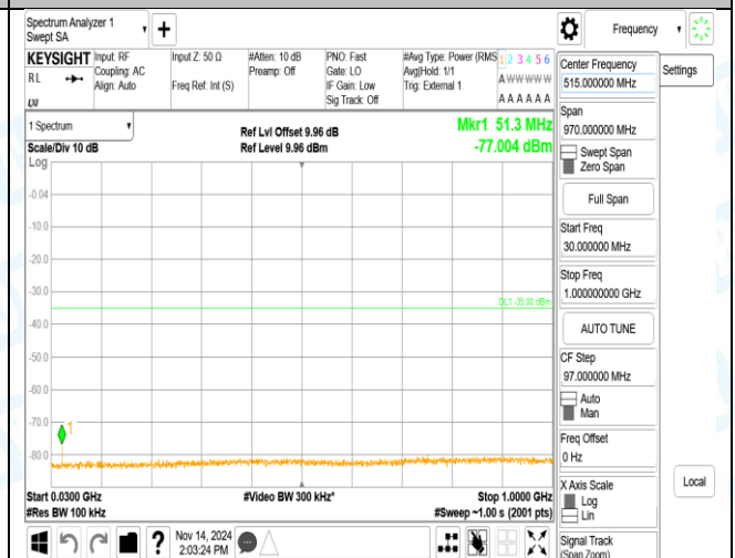
Band41_10MHz_16QAM_40090_1RB#0_20000~27000_20000~27000
