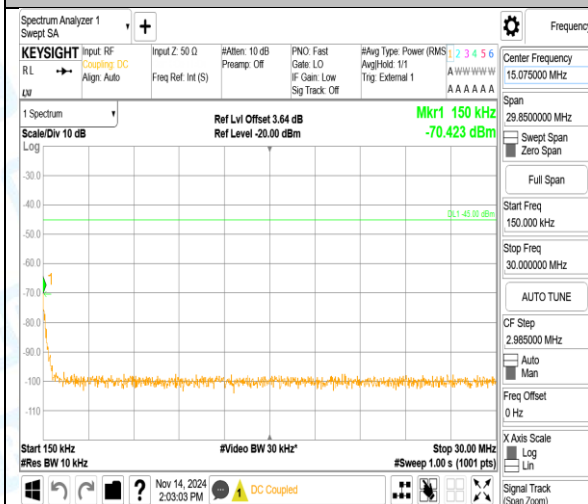
Band41_10MHz_16QAM_40090_1RB#0_1000~20000_1000~20000
