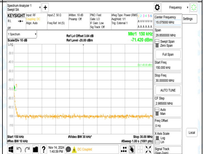
Band41_5MHz_16QAM_40590_1RB#0_1000~20000_1000~20000
