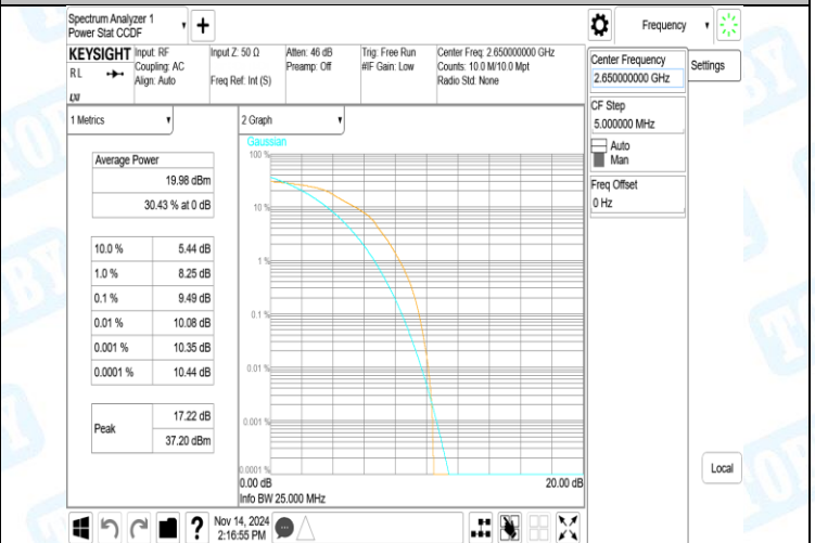
41(2535-2655)-15MHz-QPSK-40115-75RB#0-PASS
