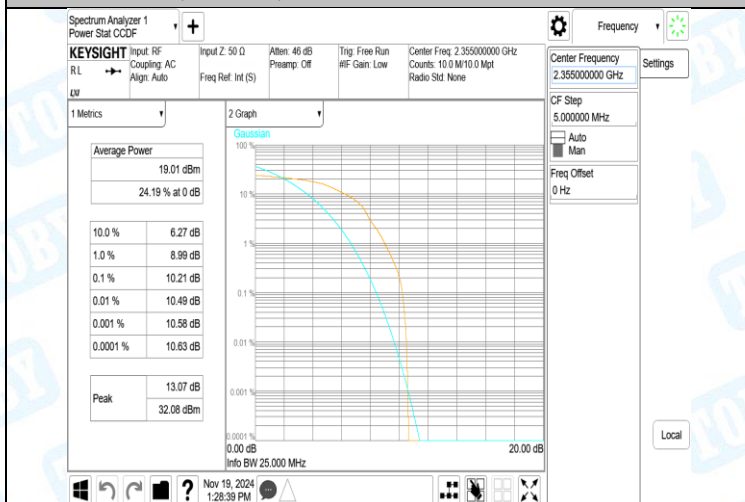
40(2350-2360)-5MHz-16QAM-39225-1RB#0-PASS
