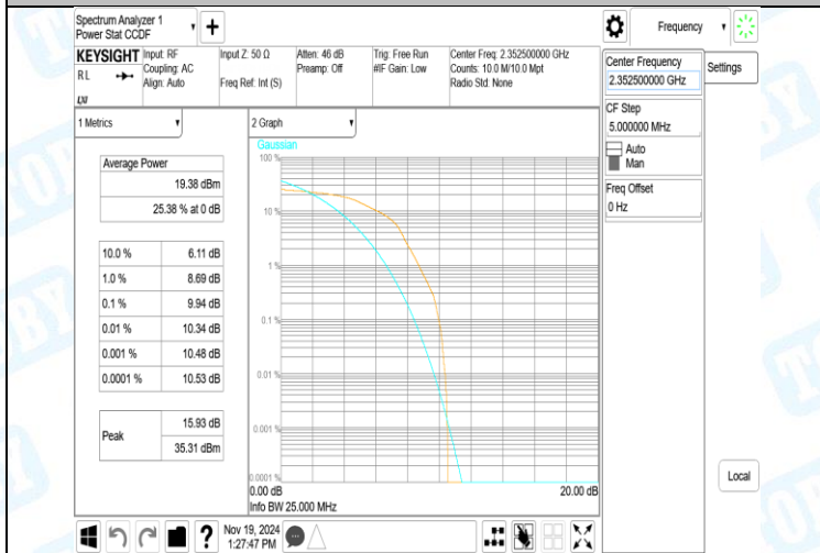
40(2350-2360)-5MHz-16QAM-39200-1RB#0-PASS
