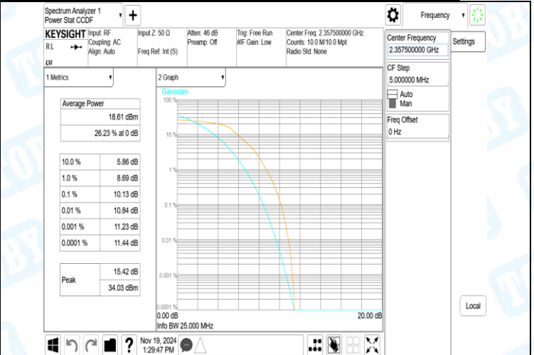
40(2350-2360)-5MHz-16QAM-39175-25RB#0-PASS
