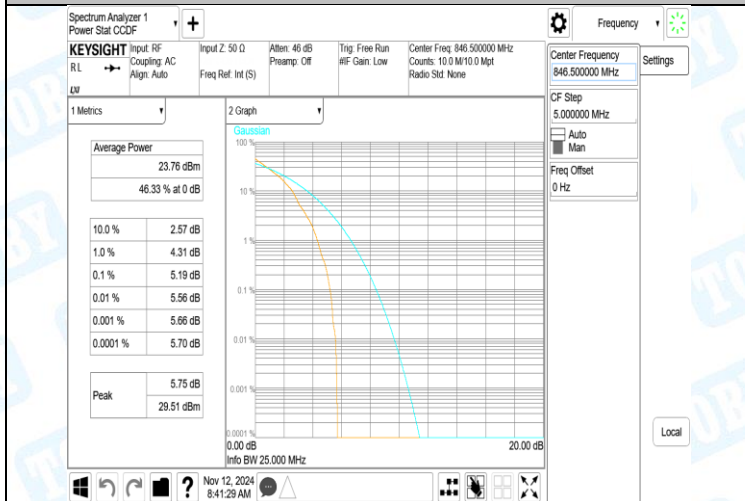
Band5-5MHz-16QAM-20425-1RB#0-PASS
