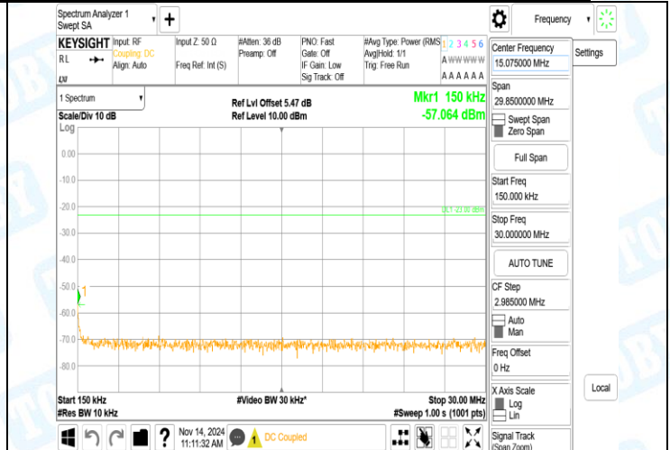
Band5-4132-5-0.15~30MHz-PASS
