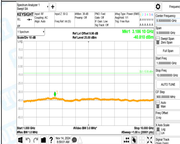
Band5-4182-3-1000~10000MHz-PASS
