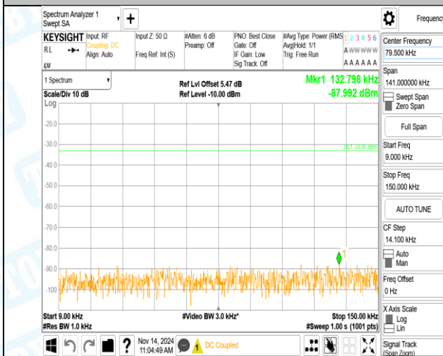
Band5-4182-3-0.009~0.15MHz-PASS
