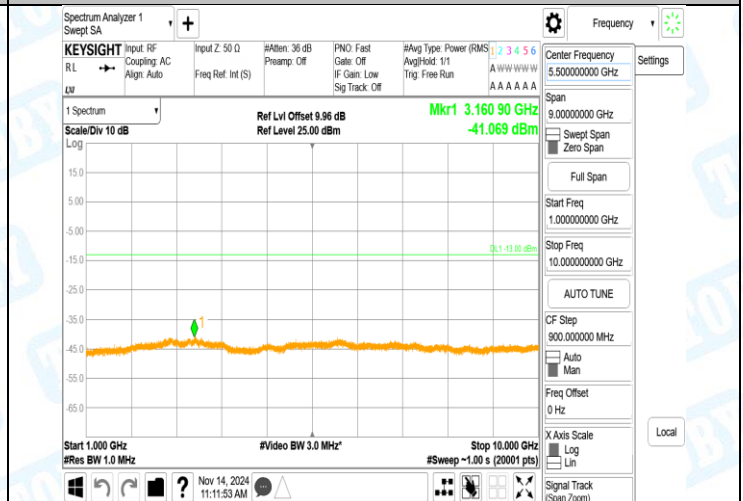
Band5-4132-5-1000~10000MHz-PASS
