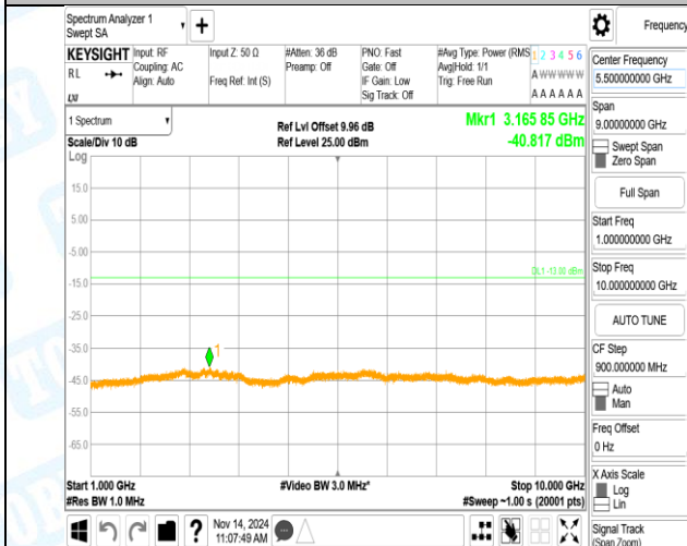
Band5-4132-4-1000~10000MHz-PASS
