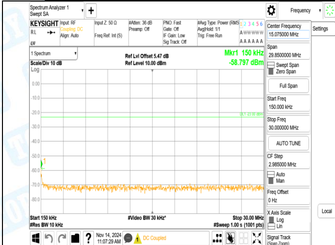
Band5-4132-4-0.15~30MHz-PASS
