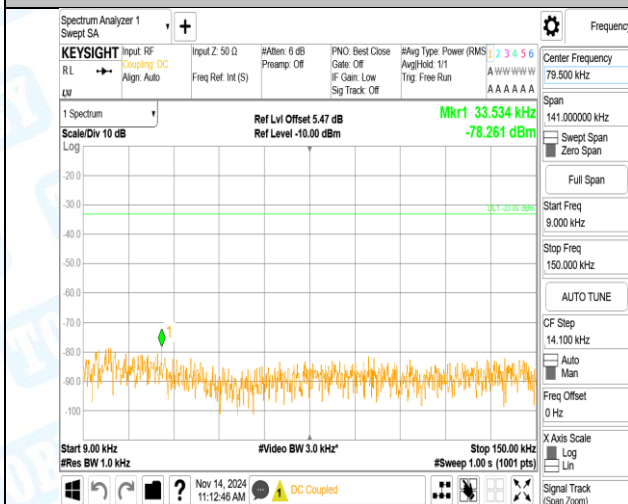
Band5-4182-5-0.009~0.15MHz-PASS
