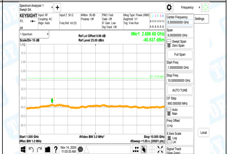
Band5-4132-3-1000~10000MHz-PASS
