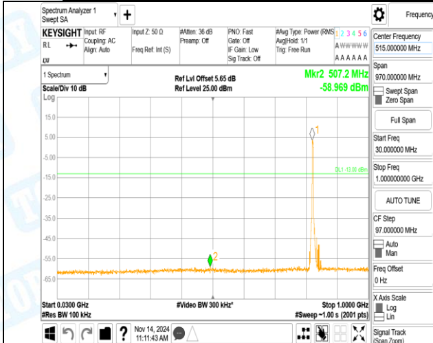
Band5-4132-5-30~1000MHz-PASS
