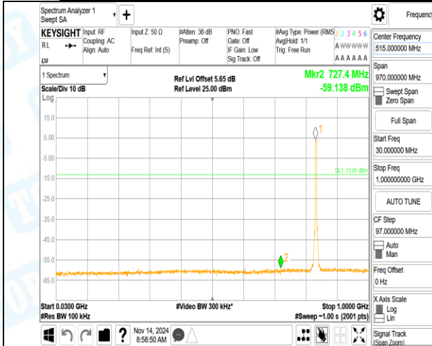
Band5-4182-3-30~1000MHz-PASS
