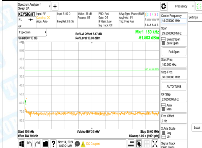
Band5-4233-3-0.15~30MHz-PASS
