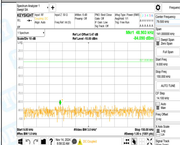
Band5-4182-3-0.009~0.15MHz-PASS
