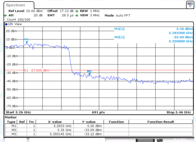
11AC40SISO-Ant1-5310-PASS
