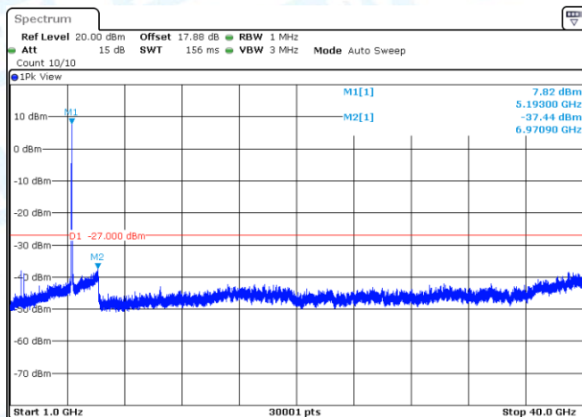
11AC40SISO-Ant1-5190-1000~40000-PASS
