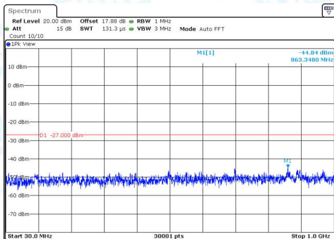
11AC40SISO-Ant1-5190-30~1000-PASS
