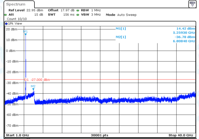
11N20SISO-Ant1-5260-1000~40000-PASS
