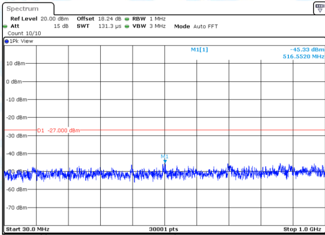
11AC20SISO-Ant1-5785-30~1000-PASS
