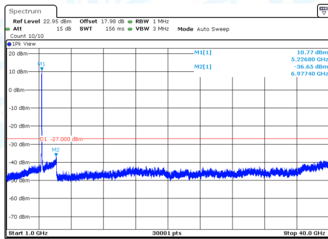
11N40SISO-Ant1-5190-1000~40000-PASS
