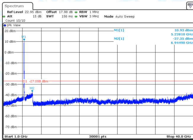
11AC40SISO-Ant1-5190-1000~40000-PASS
