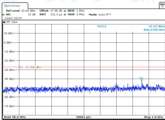
11N40SISO-Ant1-5190-30~1000-PASS
