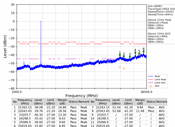
802.11ac(VHT20)_LCH_5745MHz_MIMO_NTNV
