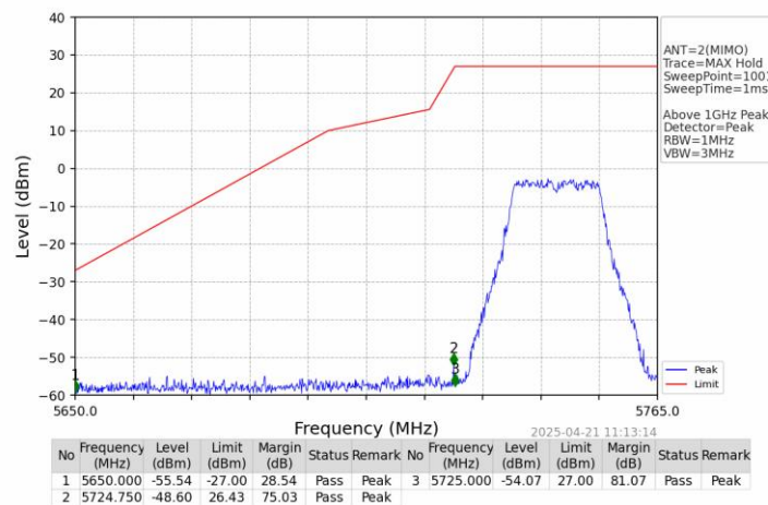
802.11ac(VHT20)_LCH_5745MHz_Ant2_NTNV
