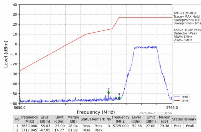
802.11ac(VHT20)_LCH_5745MHz_Ant1_NTNV
