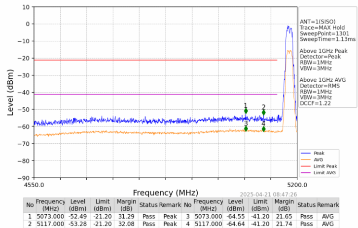
802.11a_LCH_5180MHz_Ant1_NTNV
