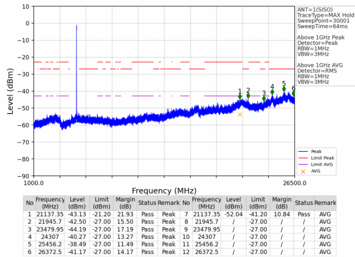
802.11a_LCH_5180MHz_Ant1_NTNV
