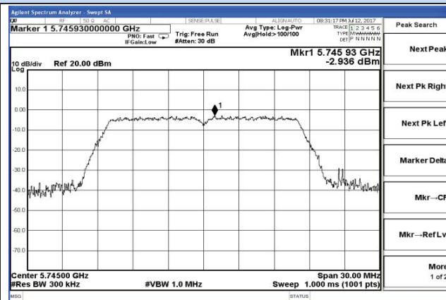
Chain 1-802.11a-5745MHz
