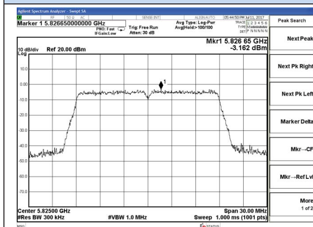
Chain 0-802.11n20-5825MHz
