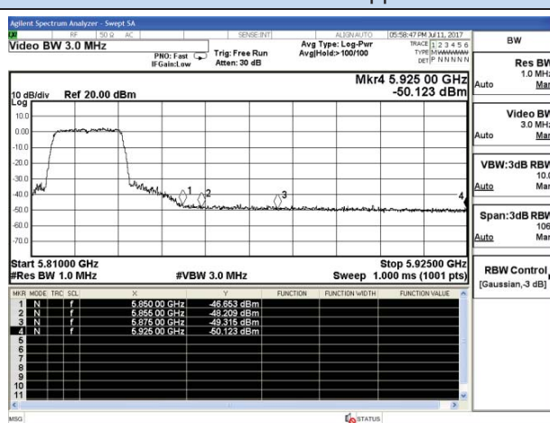
802.11n20-5825MHz-Upper
