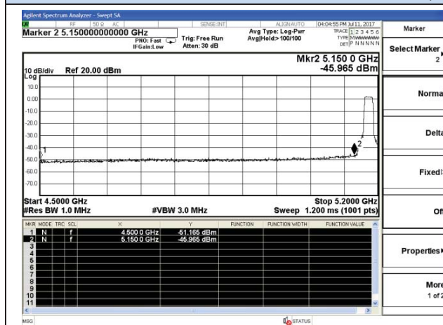
802.11a-5180MHz-Lower
