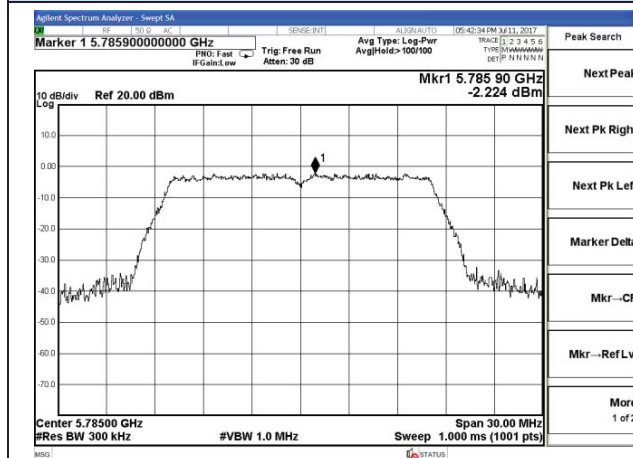
Chain 0-802.11a-5785MHz
