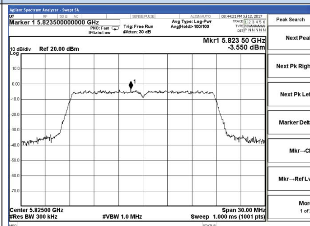
Chain 1-802.11n20-5825MHz
