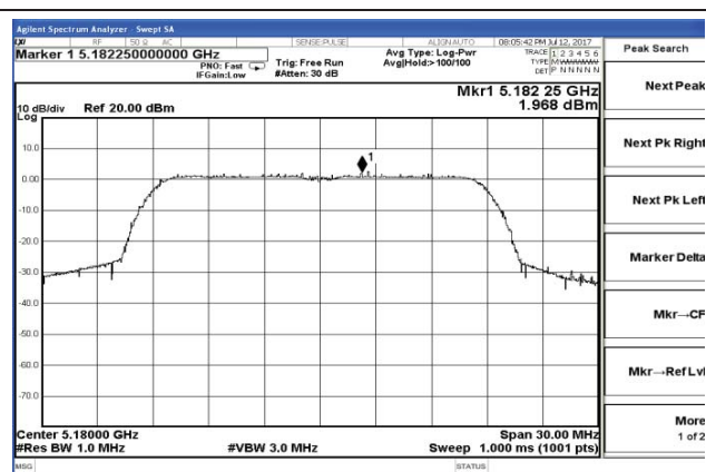
Chain 1-802.11n20-5180MHz
