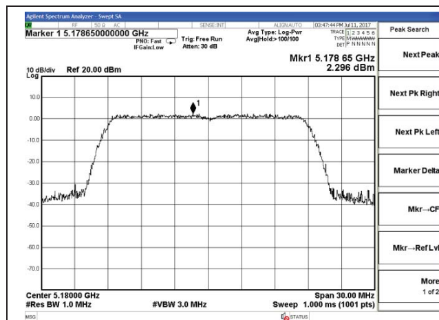
Chain 0-802.11n20-5180MHz
