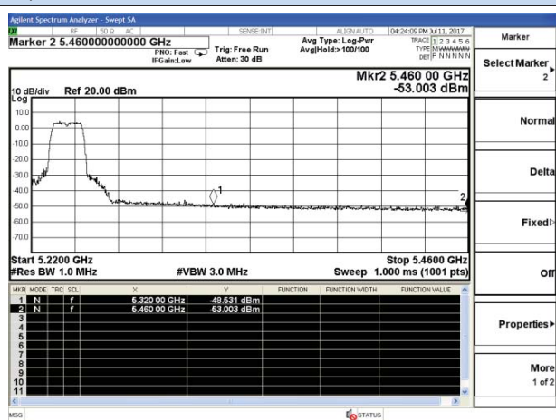
802.11a-5240MHz-Upper
