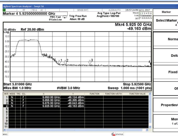
802.11a-5825MHz-Upper
