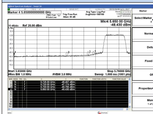
802.11n20-5745MHz-Lower
