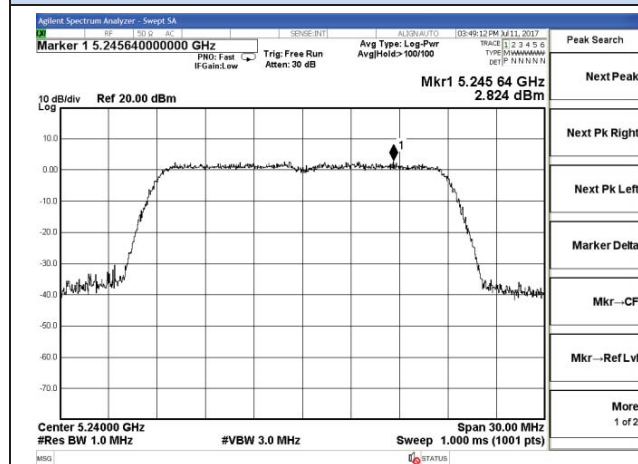
Chain 0-802.11n20-5240MHz
