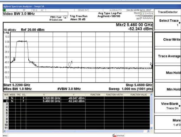
802.11n20-5240MHz-Upper
