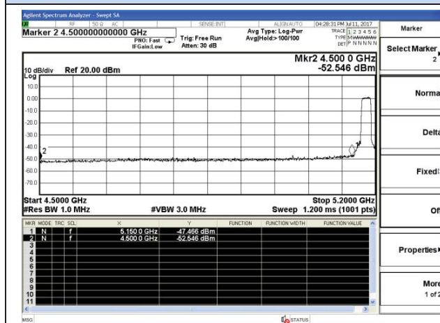
802.11n20-5180MHz-Lower
