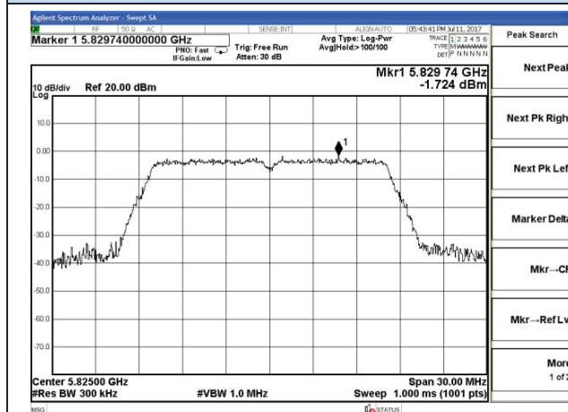
Chain 0-802.11a-5825MHz
