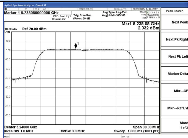
Chain 1-802.11n20-5240MHz
