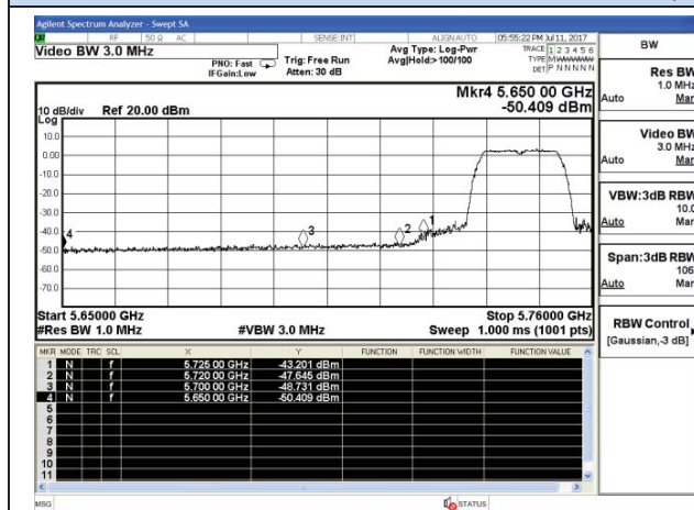
802.11a-5745MHz-Lower
