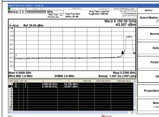
802.11n40-5190MHz-Lower
