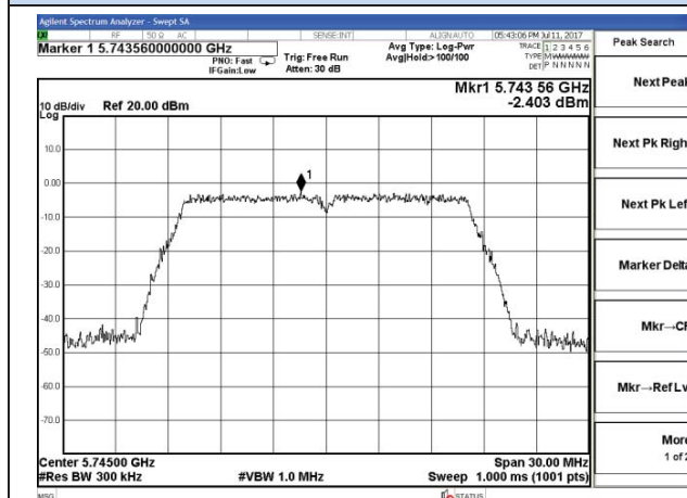
Chain 0-802.11a-5745MHz
