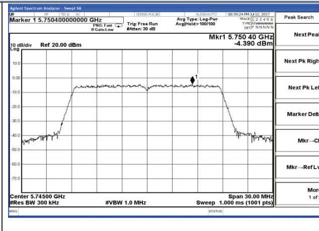
Chain 1-802.11n20-5745MHz
