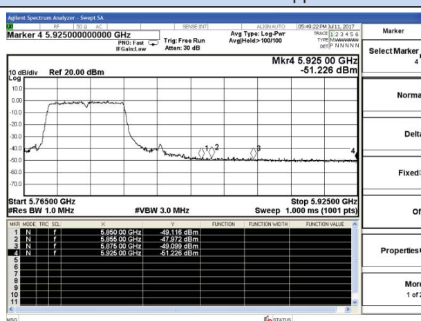
802.11n40-5795MHz-Upper
