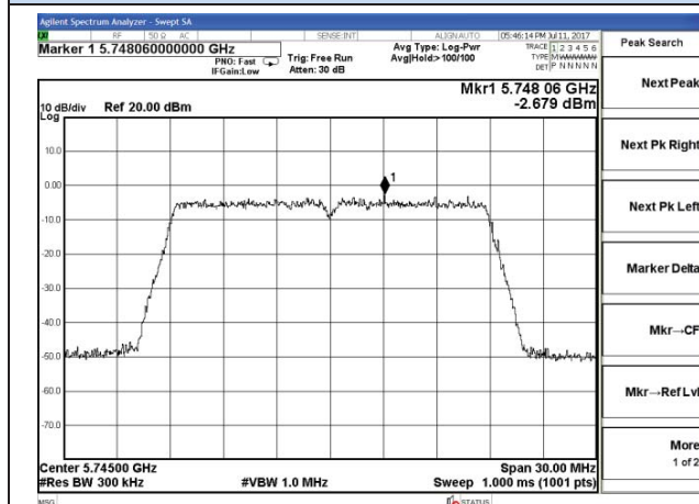
Chain 0-802.11n20-5745MHz
