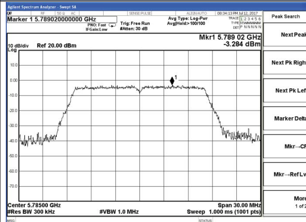
Chain 1-802.11a-5785MHz
