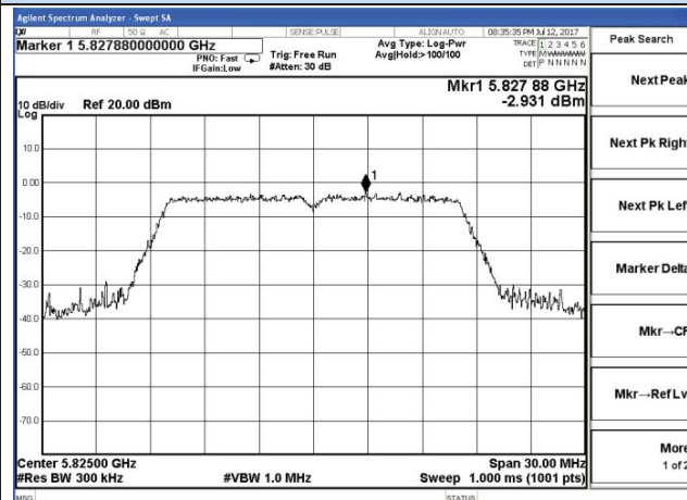
Chain 1-802.11a-5825MHz
