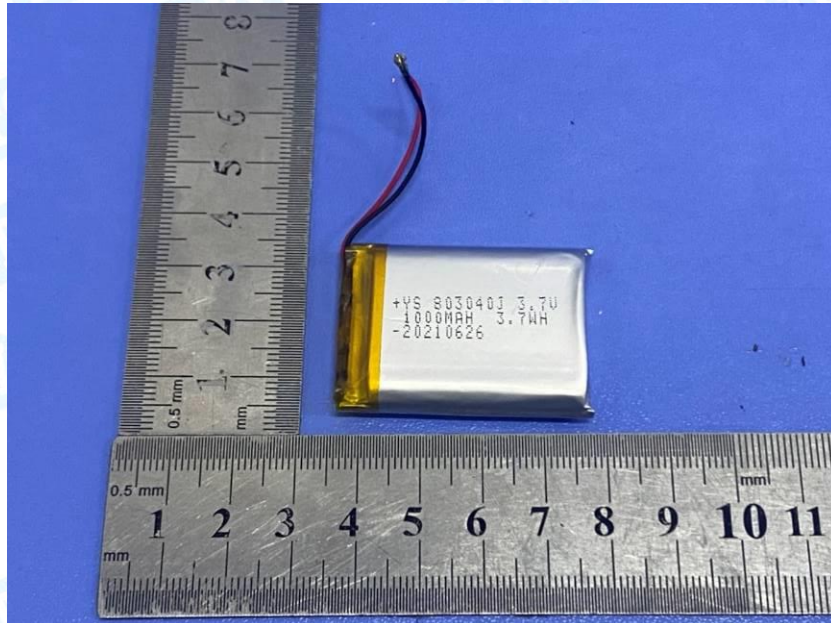
Photo 14 Appearance of Battery
