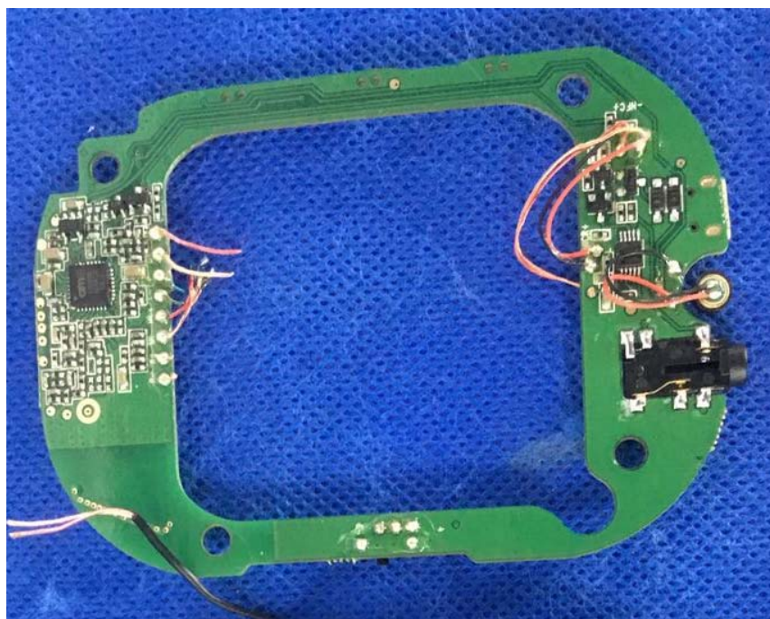
Photo 5 Appearance of PCB
