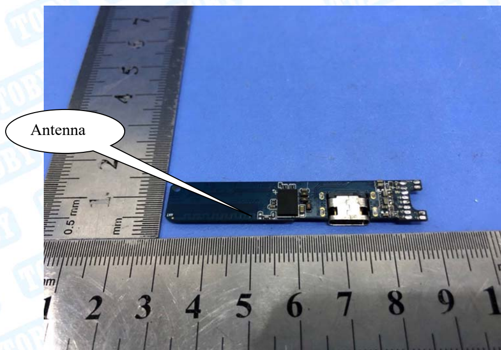
Photo 6 Internal of PCB
