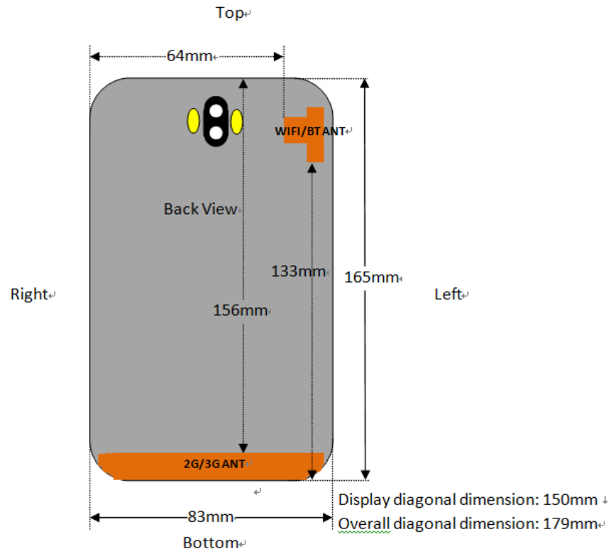
Fig.14.1 EUT Antenna Locations
