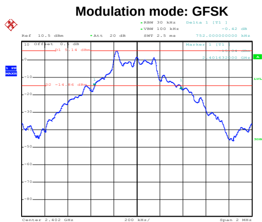
Lowest channel
