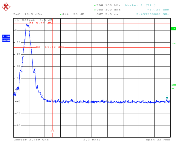
No-hopping mode
