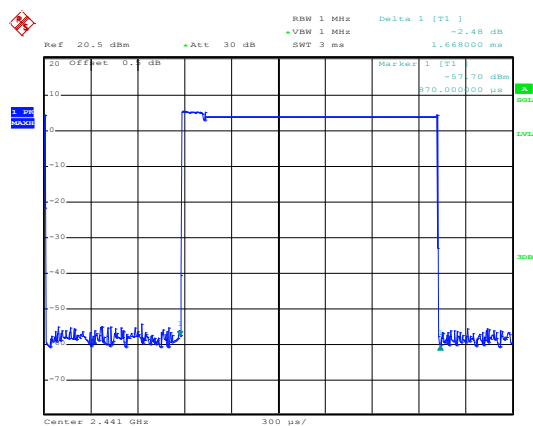
2-DH3
