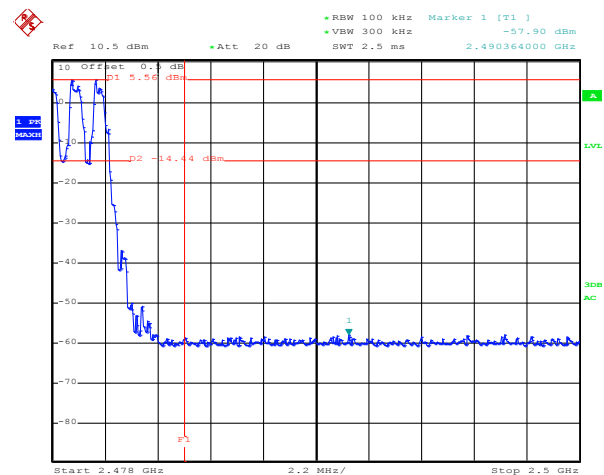
Hopping mode
