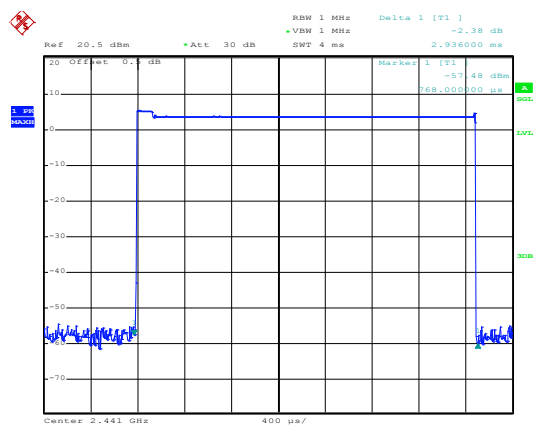
3-DH3
