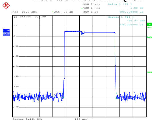
2-DH1
