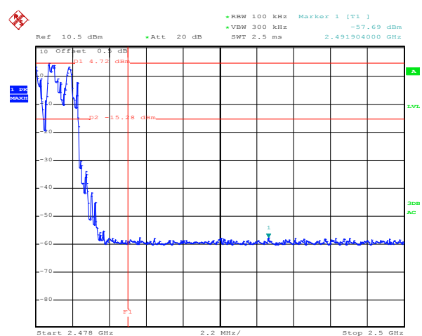
Hopping mode
