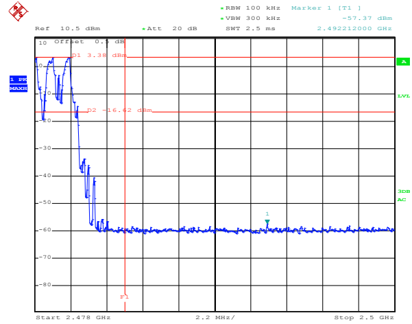
Hopping mode
