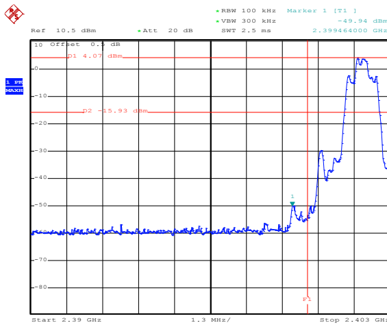
No-hopping mode
