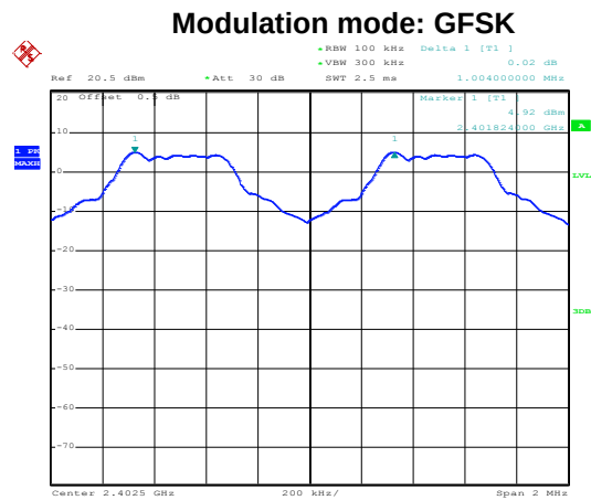
Lowest channel
