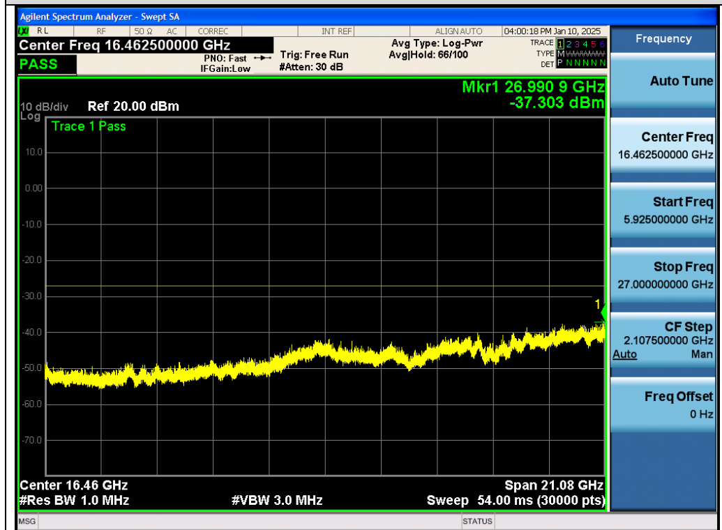
Test_Graph_802.11ac80_ANT1_5775_MCS0_Frequency Band4
