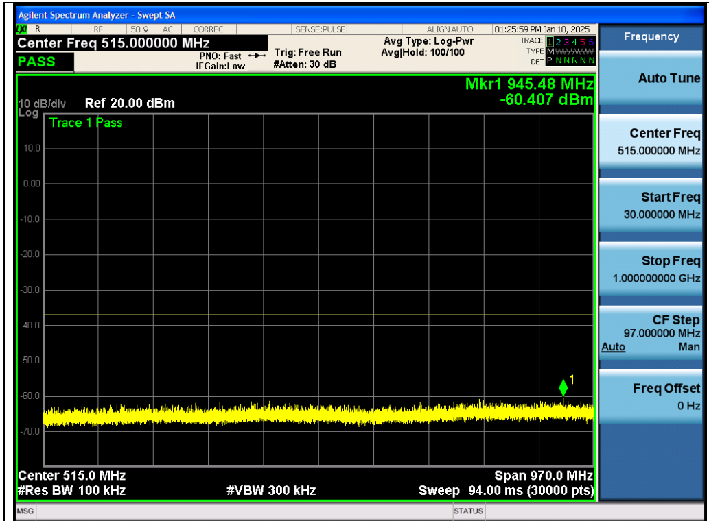
Test_Graph_802.11a_ANT1_5260_6Mbps_Frequency Band 1
