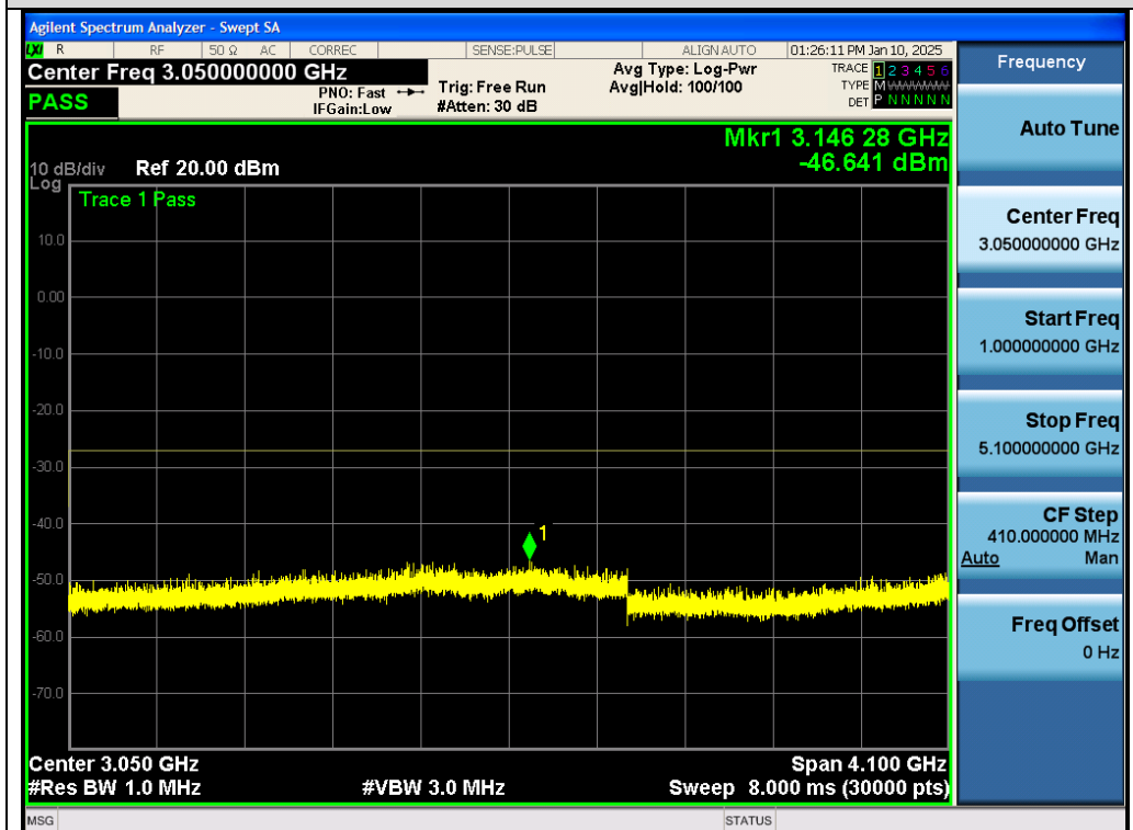
Test_Graph_802.11a_ANT1_5260_6Mbps_Frequency Band 2
