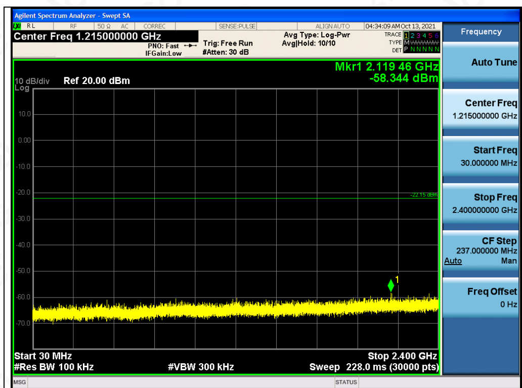
Test Graph EDR ANT1 2441 3Mbps Lower Band Emissions
