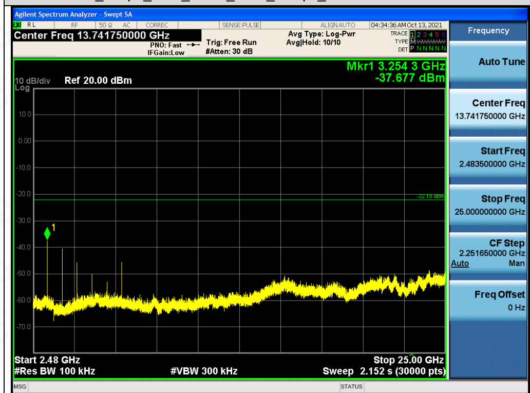
Test Graph EDR ANT1 2441 3Mbps Higher Band Emissions
