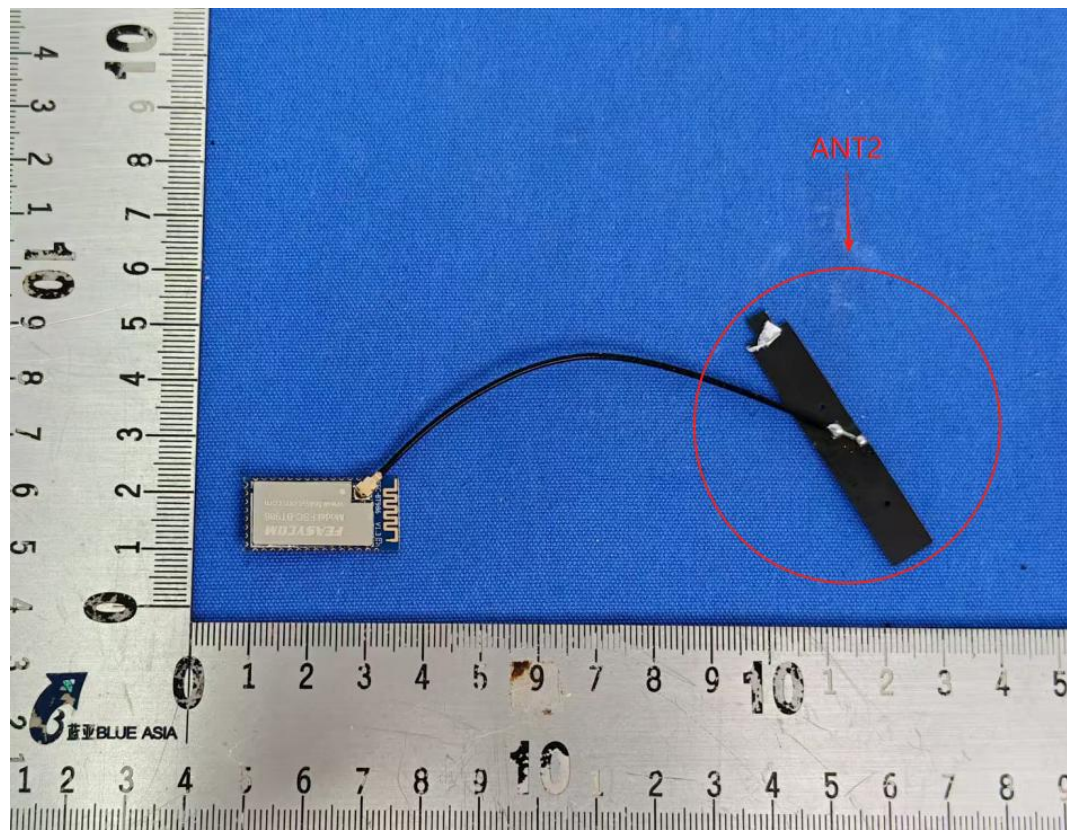
Antenna 2:
