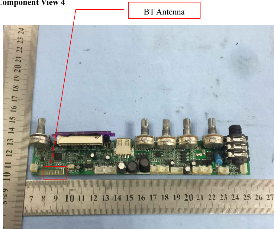
Solder Board-Component View 4
